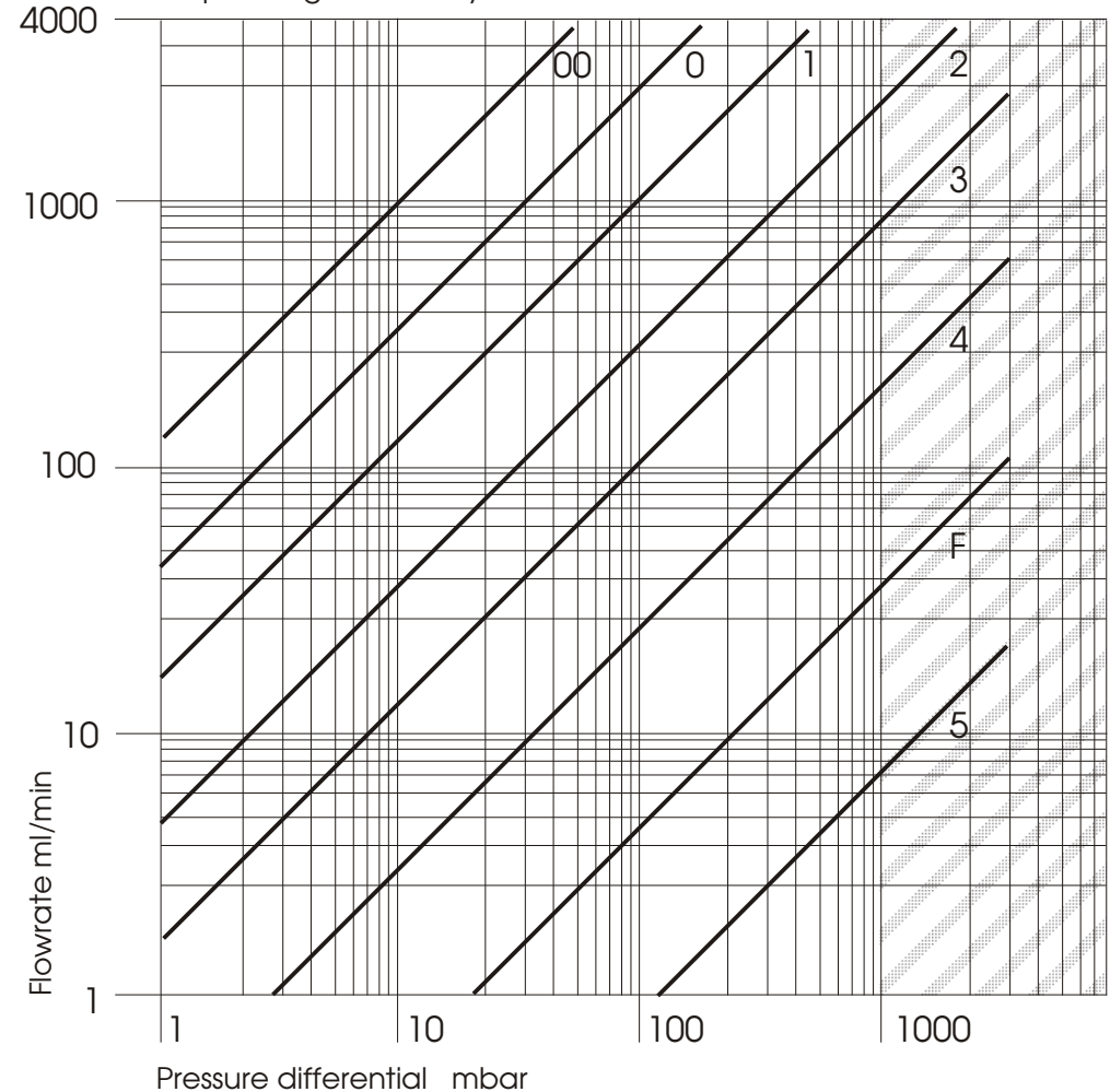
Water - Filterdisc 30 mm (at 20 deg. C) depending on Porosity Classification
