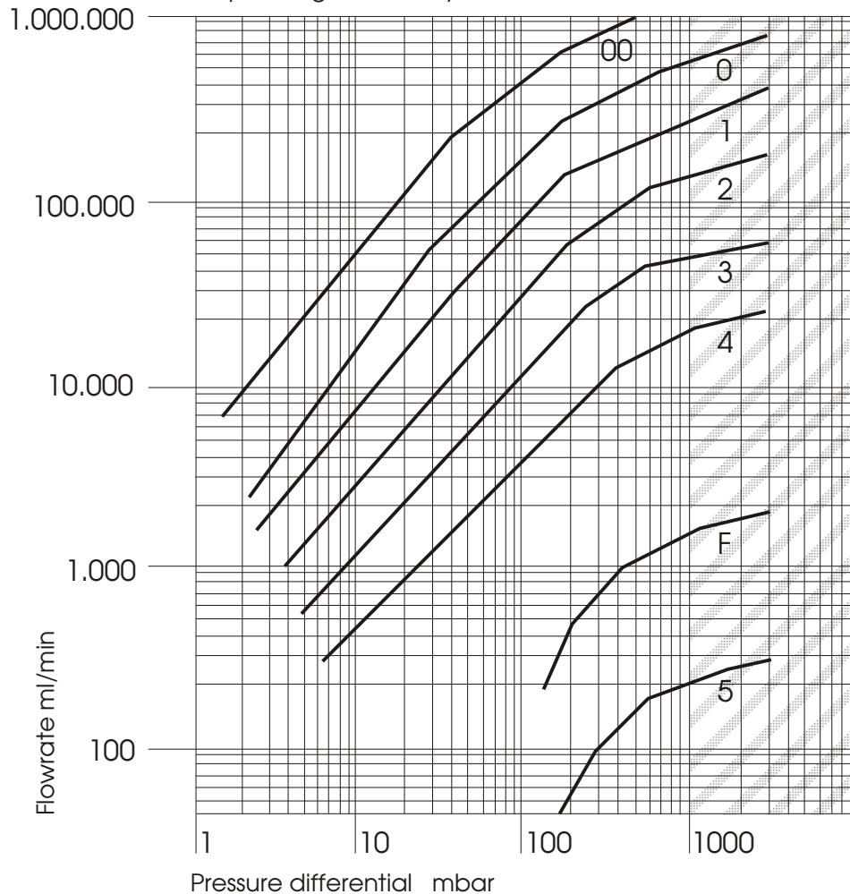
Dry Air - Filterdisc 30 mm (at 20 deg. C) depending on Porosity Classification
